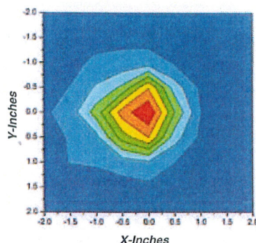
TOP INTENSITY PROFILE AT 24 IN (61 CM)
