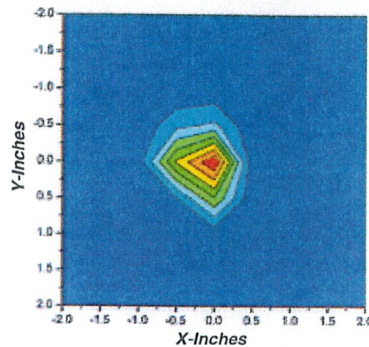
TOP INTENSITY PROFILE AT 6 IN (15 CM)
